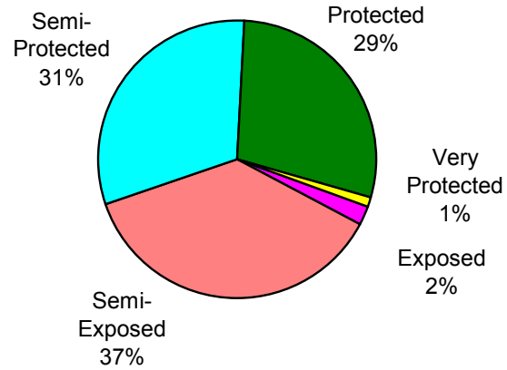
Figure 4 Wave exposure, based on observations of intertidal biota, summarized for Katmai National Park
