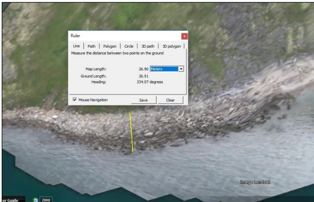
Figure 13. An Ortho-rectified image created using Structure from Motion with overlapping ShoreZone video captures. They are exported to Google Earth for width measurements of the intertidal shoreline.
