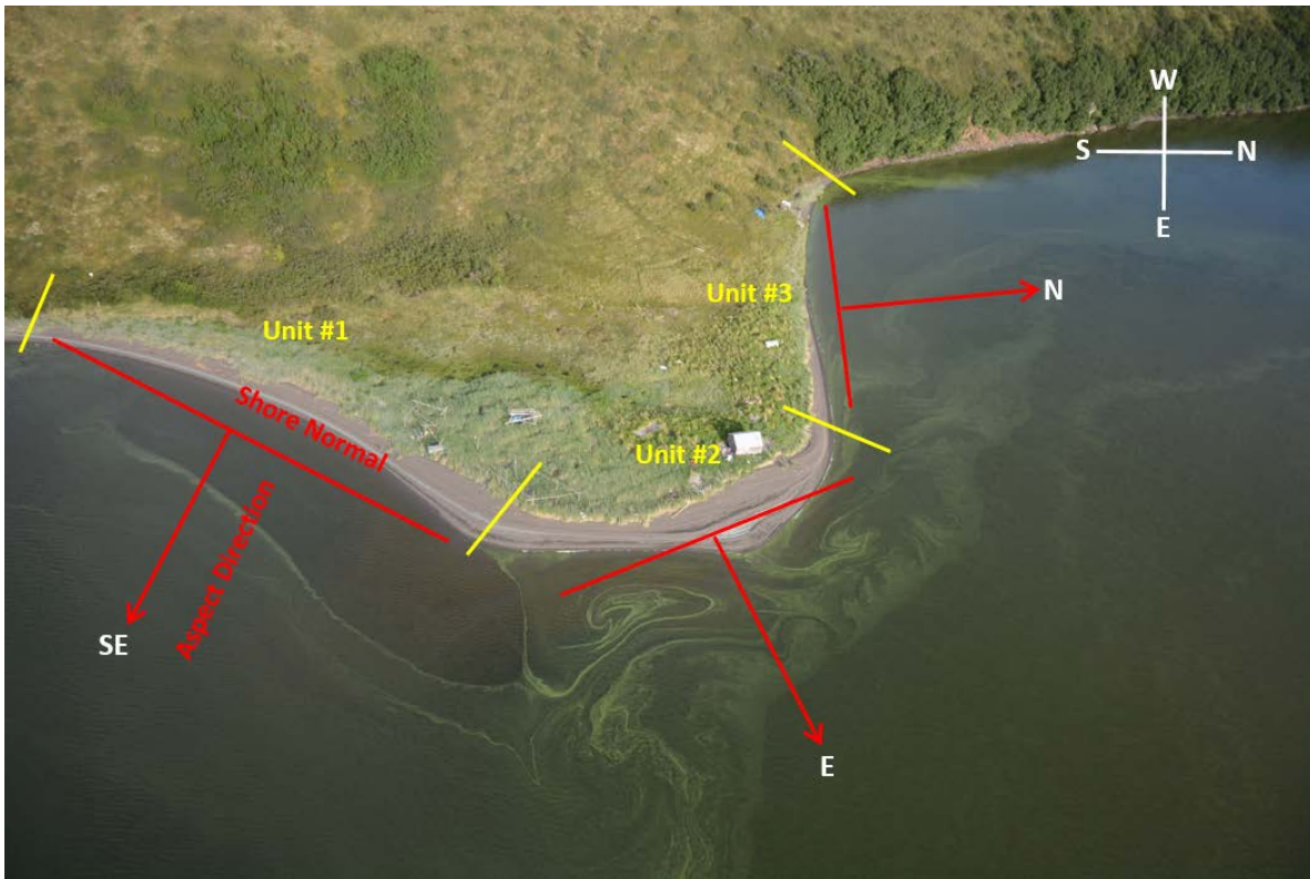
Figure 14. Determining the Aspect attribute of each alongshore Unit.
