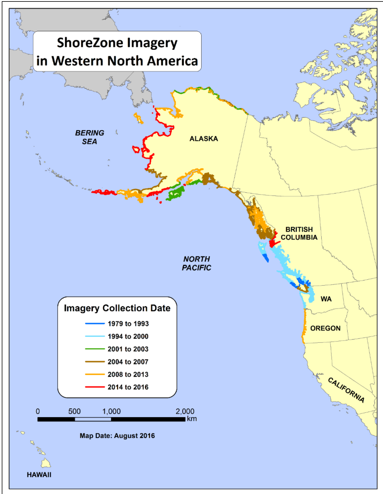
Figure 2. Chronology of ShoreZone imagery acquisition.
