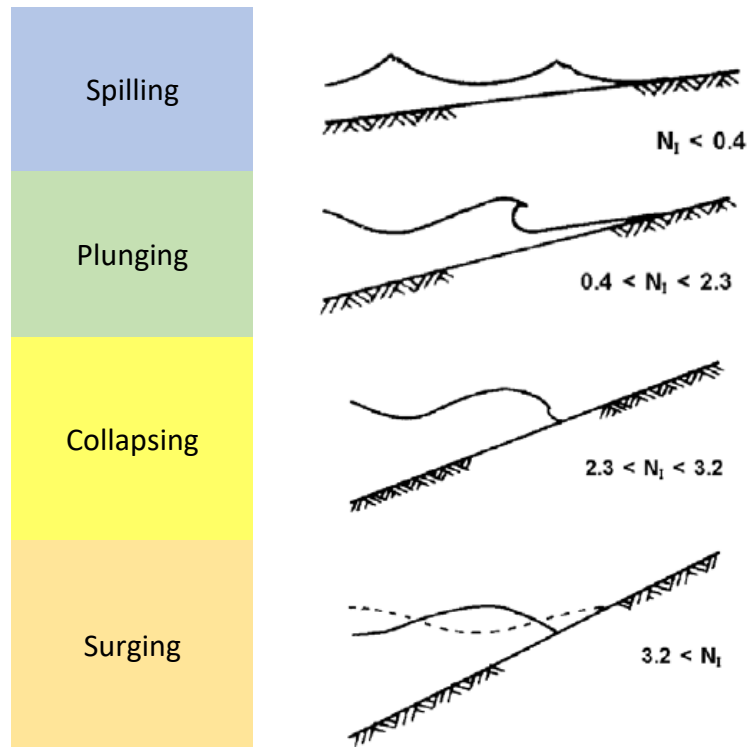
Figure 15. Illustration of the type of wave morphology represented by each Iribarren Category (after Komar 1998).
