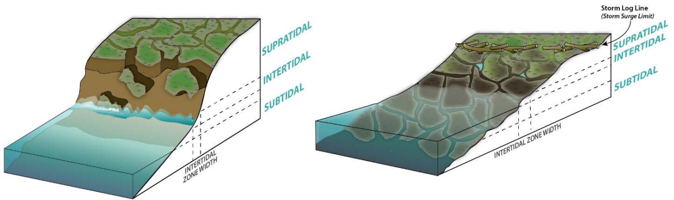
Figure 11. Examples of eroding tundra cliff (left) and inundated tundra (right) typical of those on Arctic coasts in Alaska. Note that the intertidal zone widths are often narrow, while storm surge extent may be very wide.
