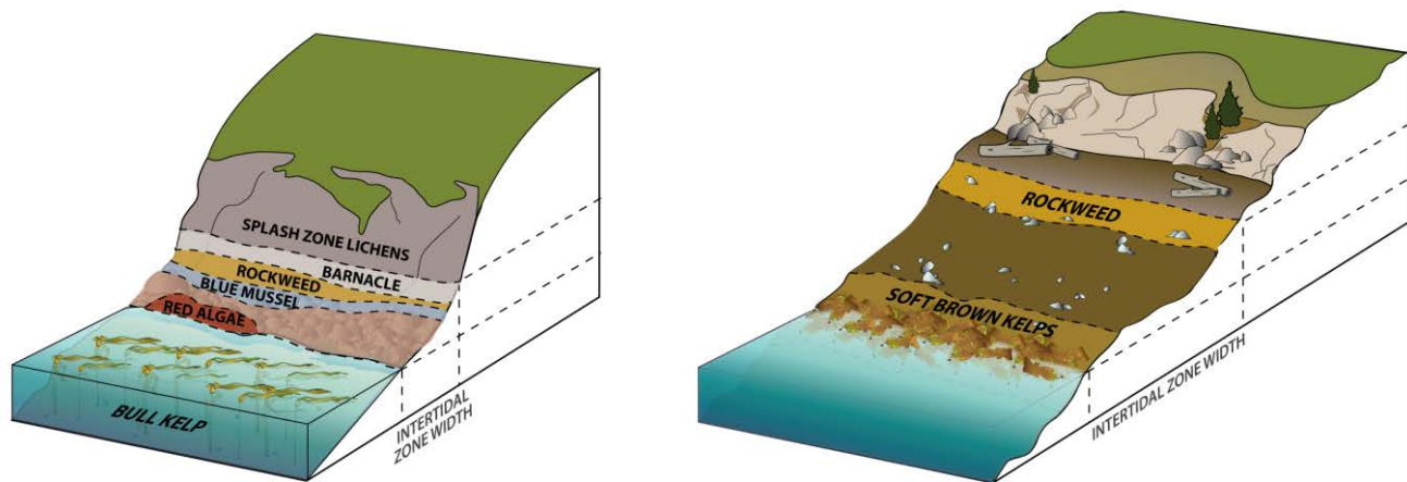
Figure 18. Typical Bioband combinations on a rocky shore (left) and a sediment shore (right).
