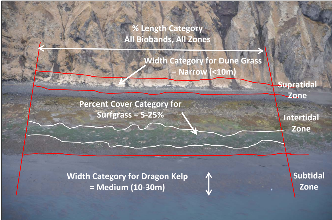
Figure 19. Illustration of the width metric for the supratidal Biobands not under the Splash Zone (SPZO) primary category and the subtidal Biobands, and the percent cover metric for intertidal Biobands.
