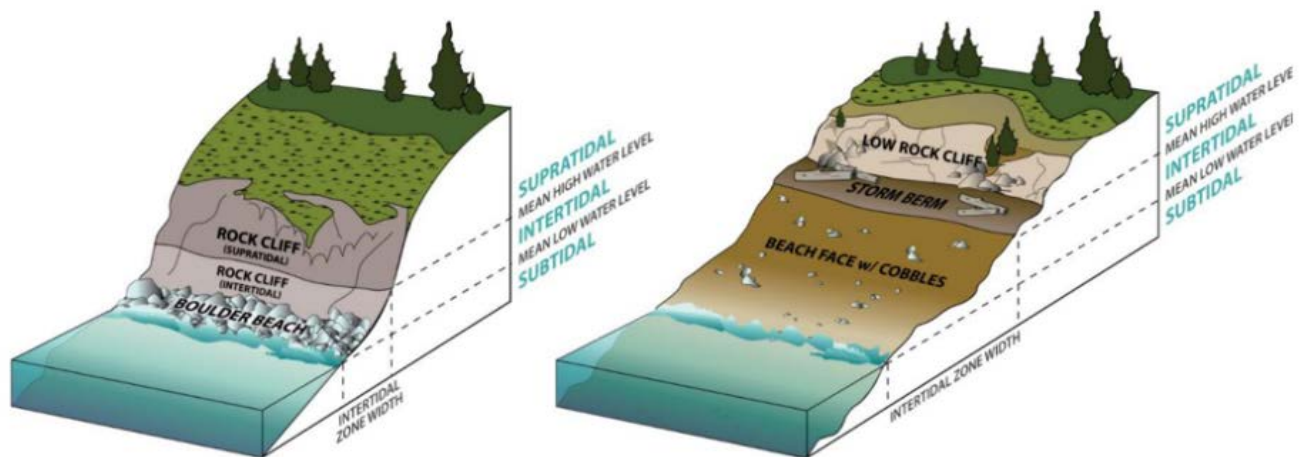
Figure 10. Across-shore zones and components on a steep (left panel) and moderately inclined (right panel) shoreline.
