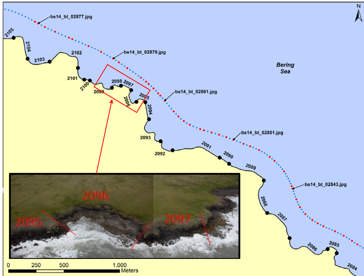
Figure 8. Example of the delineation of the digital shoreline of Nunivak Island in the Bering Sea. The inset shows a mosaic of the high resolution digital still images of the section of shoreline highlighted by the red box, with the corresponding Unit breaks shown on the photos. The blue dots show the helicopter flight line with each dot representing a 1-second positional fix for the video imagery and the red dots showing the photo locations.
