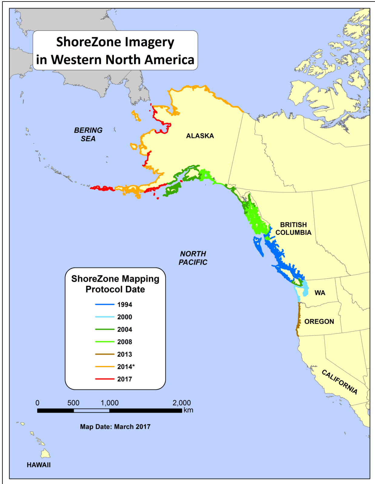
Figure 3. ShoreZone mapping associated with each protocol listed in Table 1.
