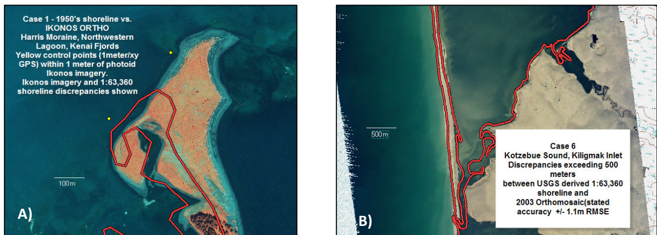
Figure 9. Discrepancies between the Coast 63 digital shoreline and satellite imagery for two National Parks in Alaska. A) shows Kenai Fjords and B) shows Kotzebue Sound.
