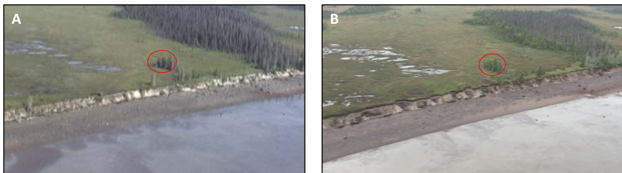
Figure 4. A) Video image taken during a ShoreZone survey in 2001 near Polly Creek in Cook Inlet. B) The same section of coast imaged during a ShoreZone survey in 2009. The red circles indicate a point of reference between the photos. It can clearly be seen that the supratidal cliff eroded in the 8 years between the surveys due to the loss of trees that were at the edge of the cliff in 2001.
