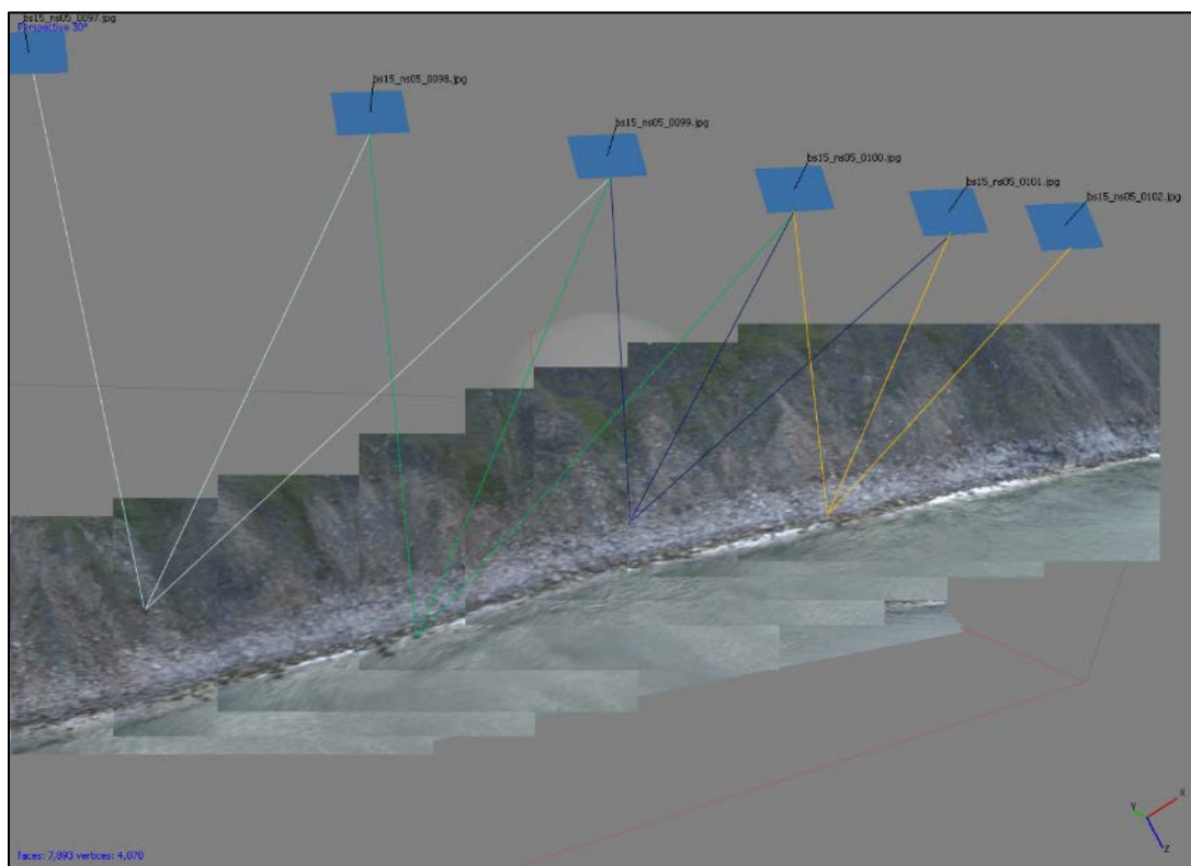
Figure 12. The Structure from Motion processing technique for video frames with 60% overlap.
