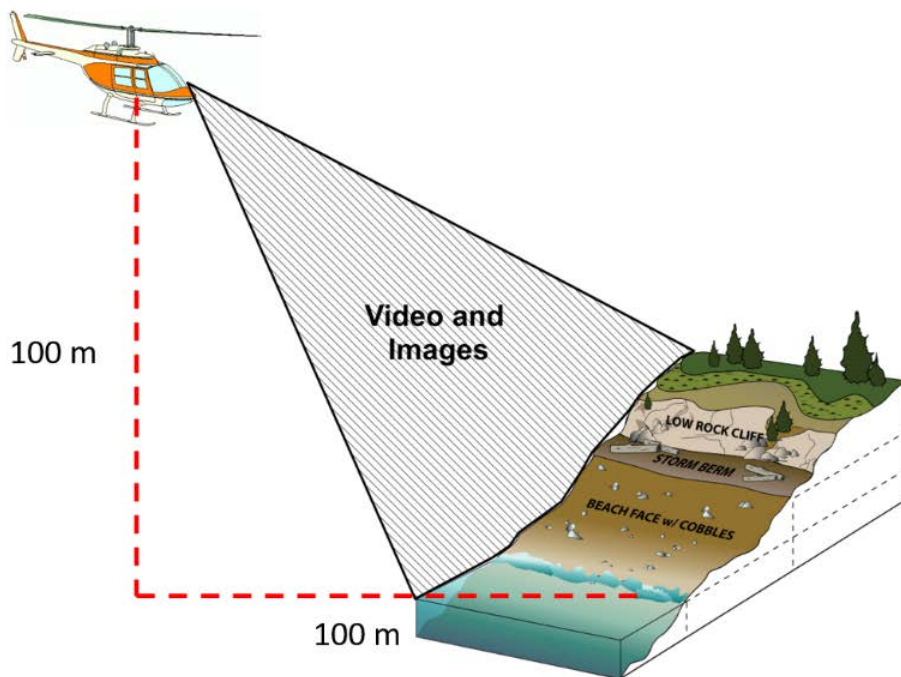
Figure 6. Oblique aerial images are acquired at 100 m altitude and 100 m offset from the shoreline leading to imagery at a 45° angle to the intertidal.
