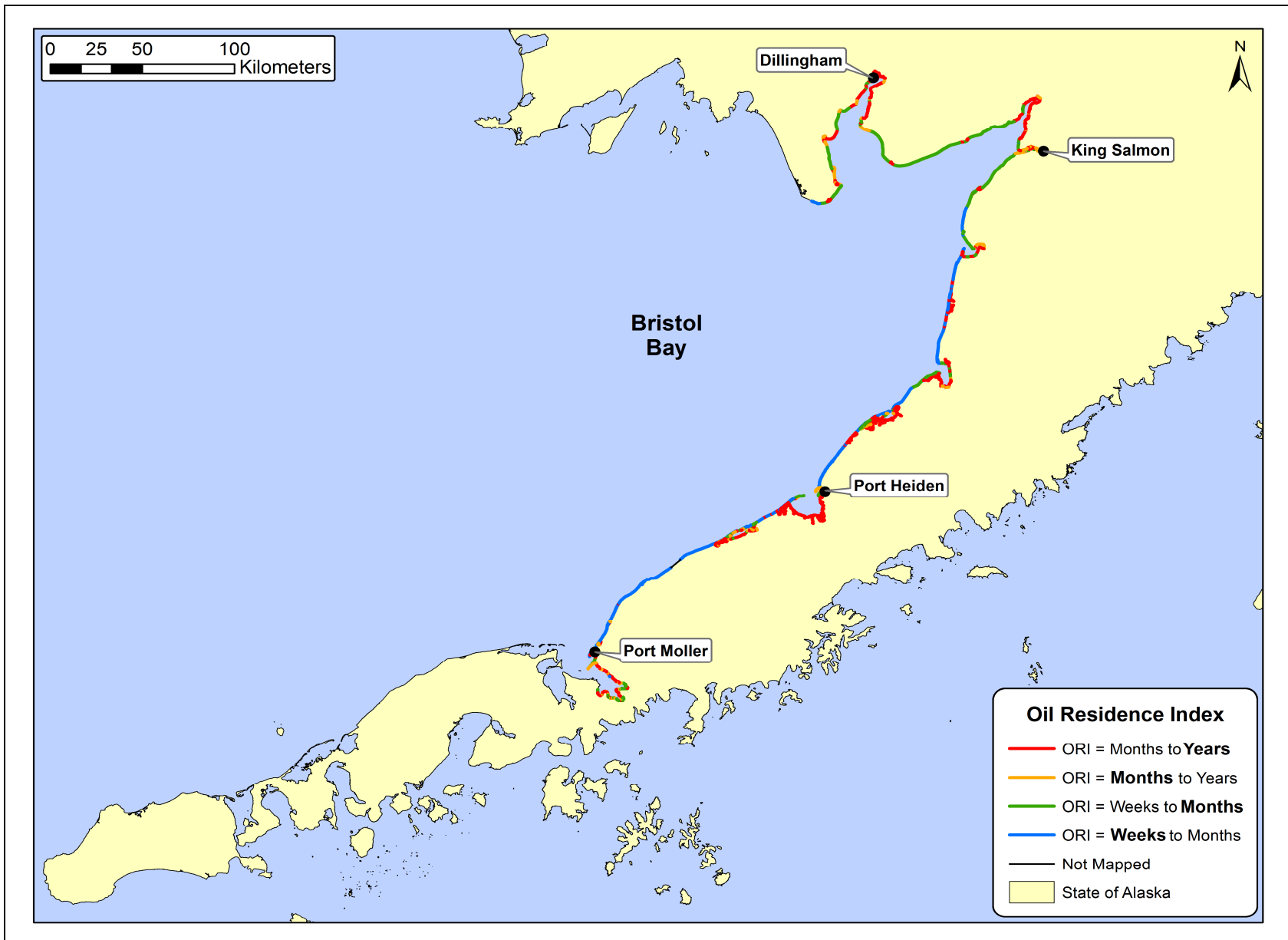
Figure 2.7. Oil Residence Index (ORI) for shorelines in Bristol Bay, based on substrate type and wave exposure (Appendix A, Table A-5).
