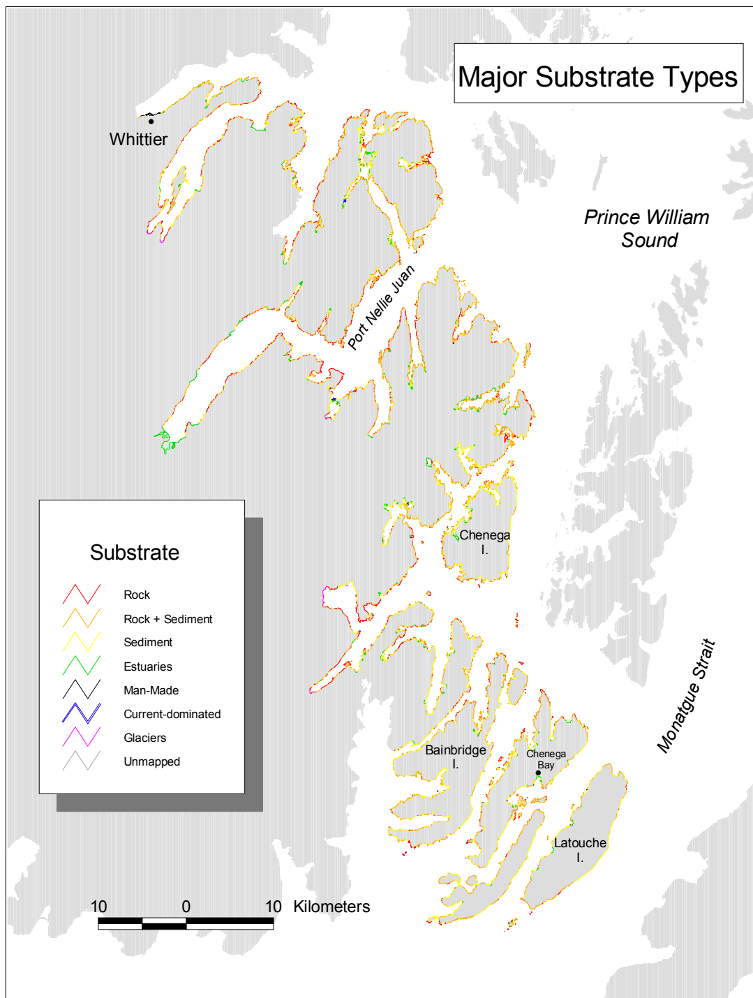
Figure 2.1. Distribution of principal substrate types (based on grouped BC Classes) in mapped areas of western Prince William Sound.
